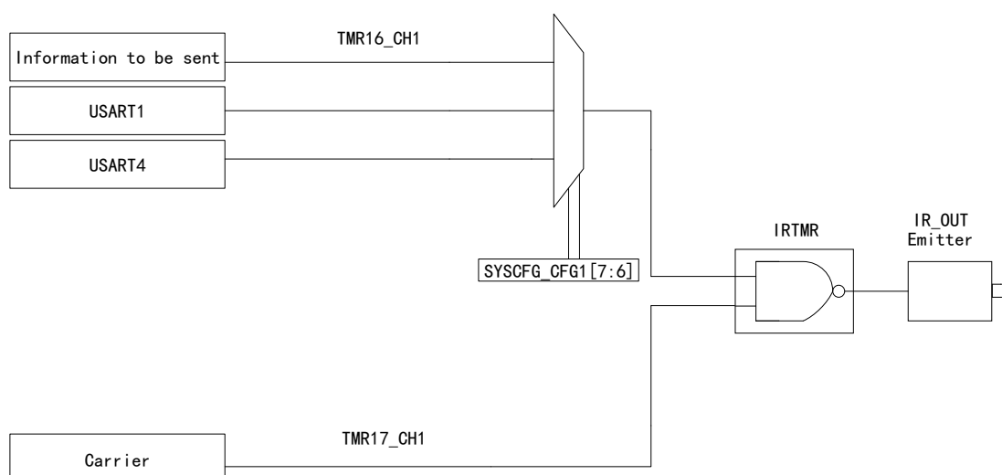
Figure 78 IRTMR Structure Block Diagram
