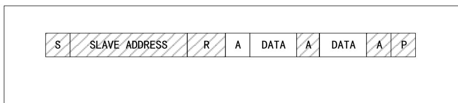
Figure 99 Master Reads Data from Slave
