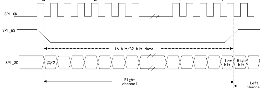
Figure 109 MSB Alignment Standard Waveform (24-bit data)
