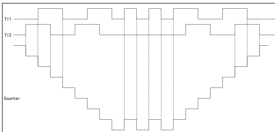
Figure 74 Example of Encoder Interface Mode of IC1FP1 Reversed Phase
