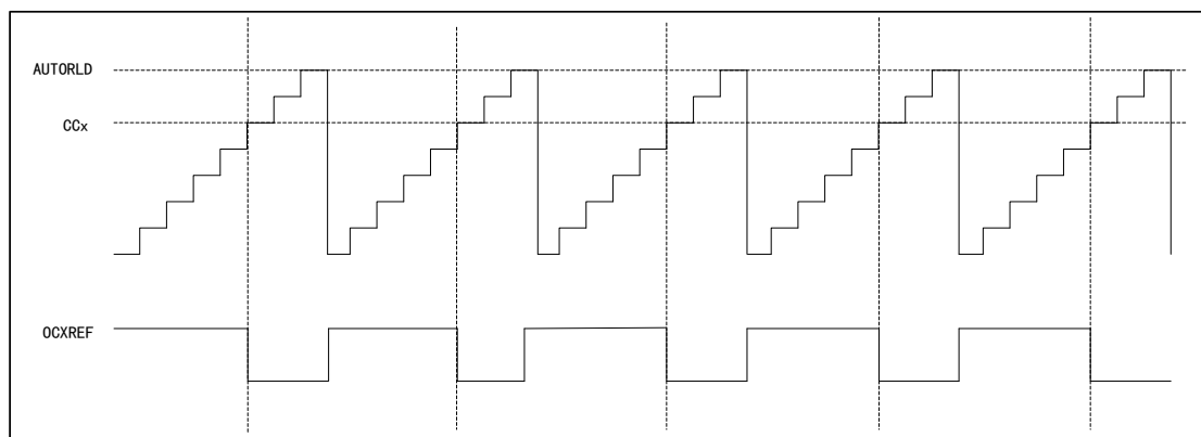
Figure 49 PWM1 Count-up Mode Timing Diagram
