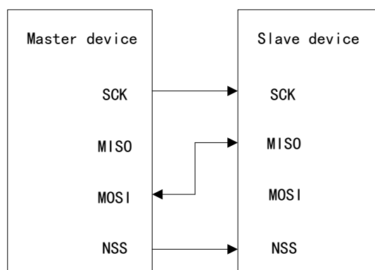
Figure 102 Connection in Half Duplex Mode
