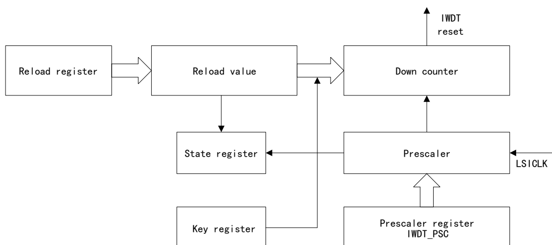
Figure 79 Independent Watchdog Block Diagram
