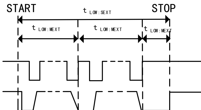
Figure 100 t_{\text{LOW:SEXT}} and t_{\text{LOW:MEXT}} Time
