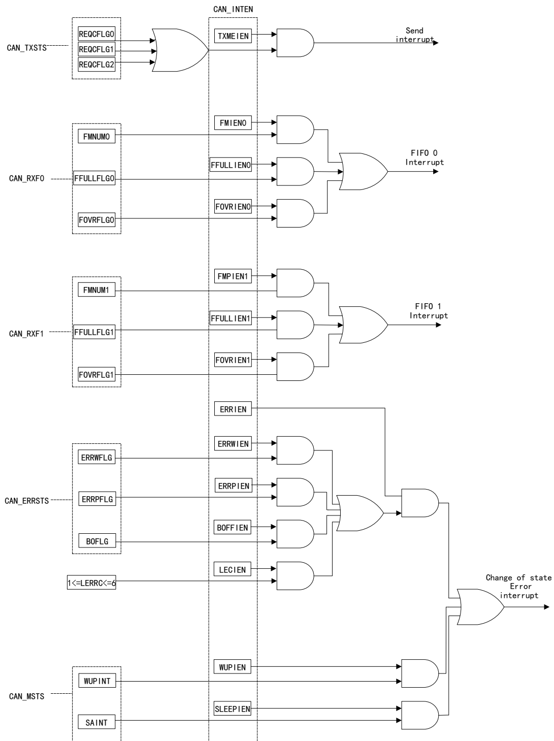
Figure 124 Event Flag and Interrupt Generation
