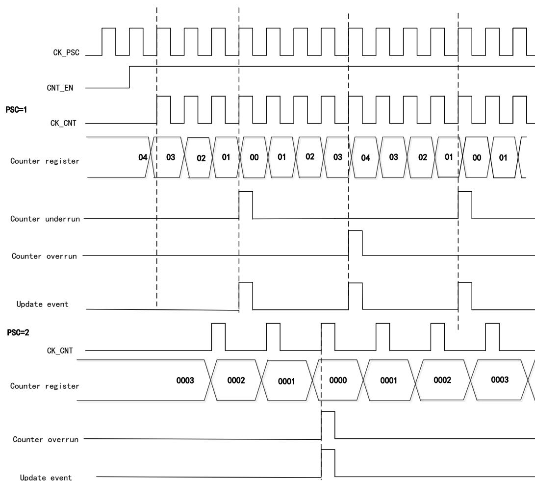
Figure 60 Timing Diagram when Division Factor is 1 or 2 in Center-aligned Mode
