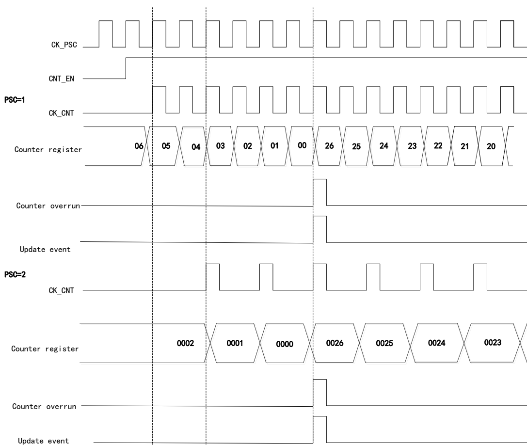
Figure 59 Timing Diagram when Division Factor is 1 or 2 in Count-down Mode
