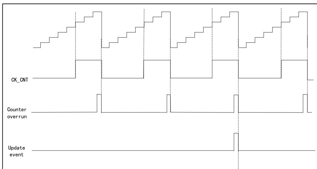
Figure 61 Timing Diagram when Setting REPCNT=2 in Count-up Mode
