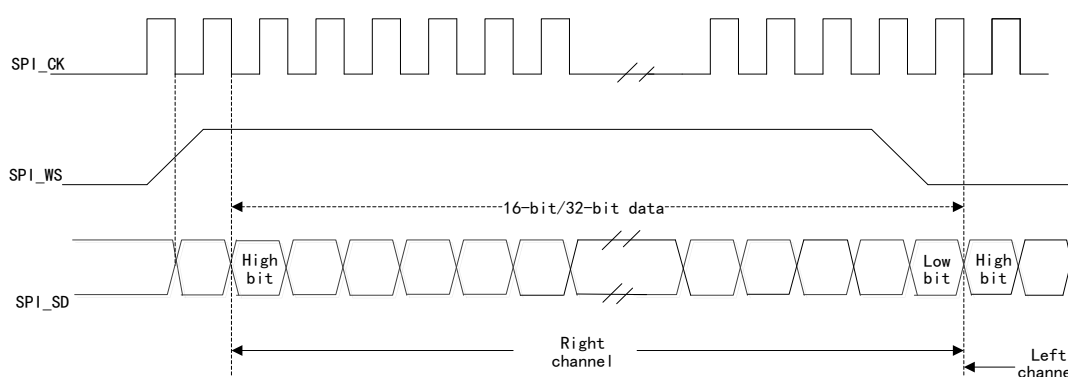
Figure 105 I2S Philips Protocol Waveform (16/32 bits)
