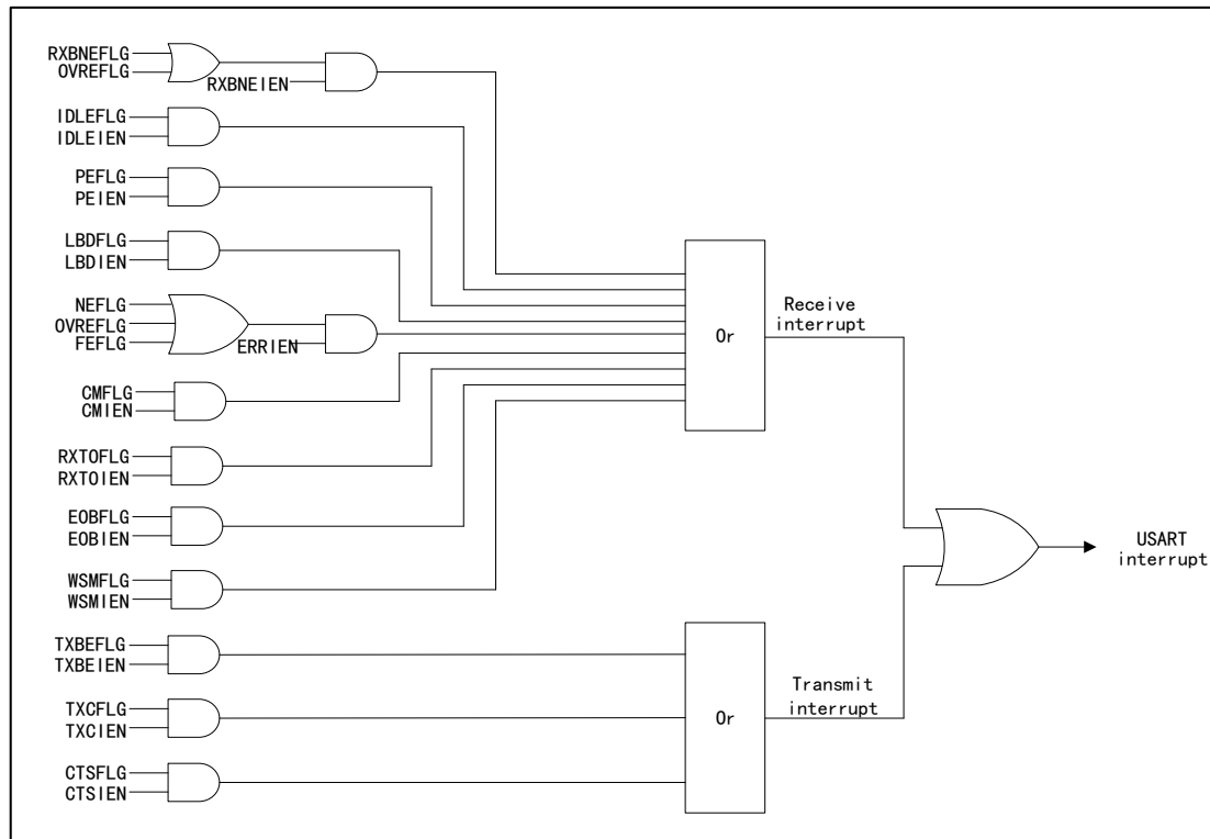
Figure 94 USART Interrupt Mapping
