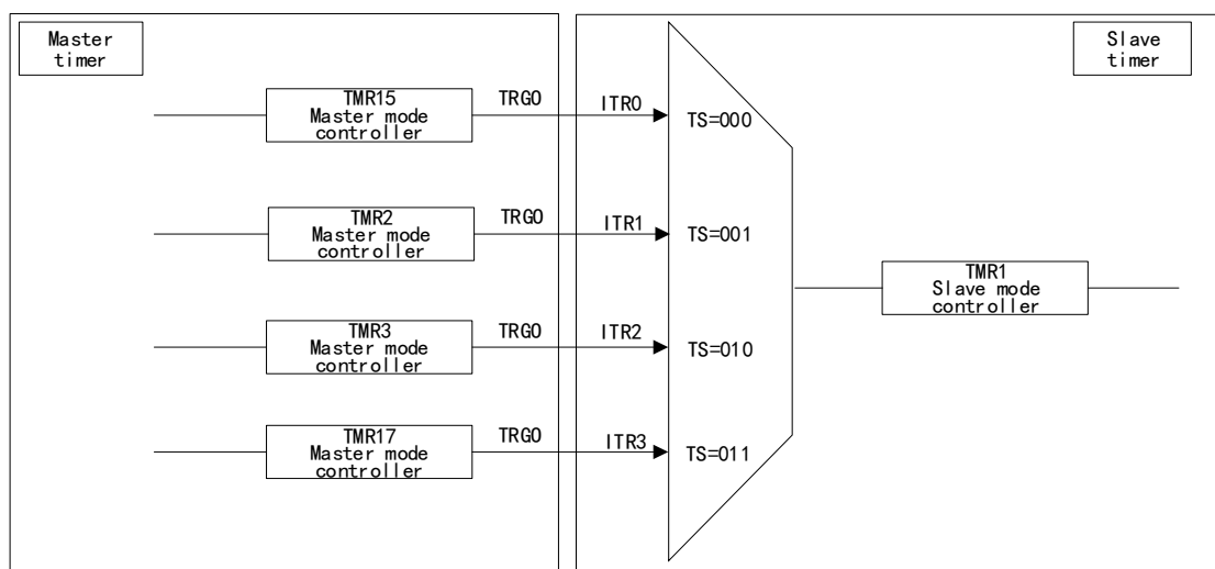
Figure 75 Timer 1 Master/Slave Mode Example
