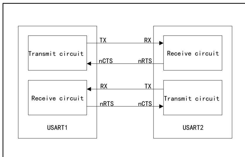
Figure 93 Hardware Flow Control between Two USARTs
