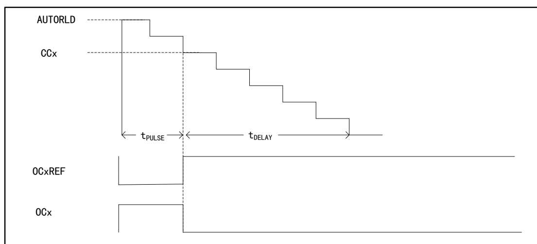
Figure 69 Single-pulse Mode Timing Diagram
