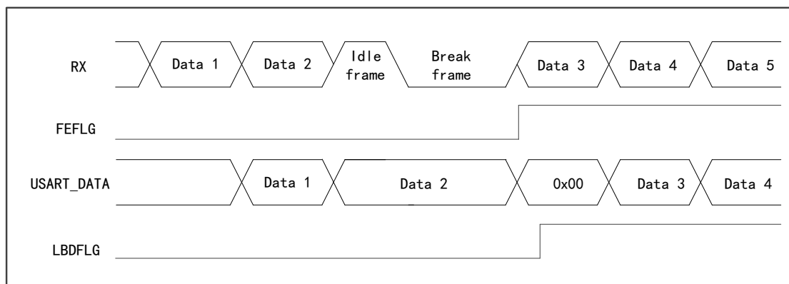
Figure 89 Break Frame Detection in Idle State
