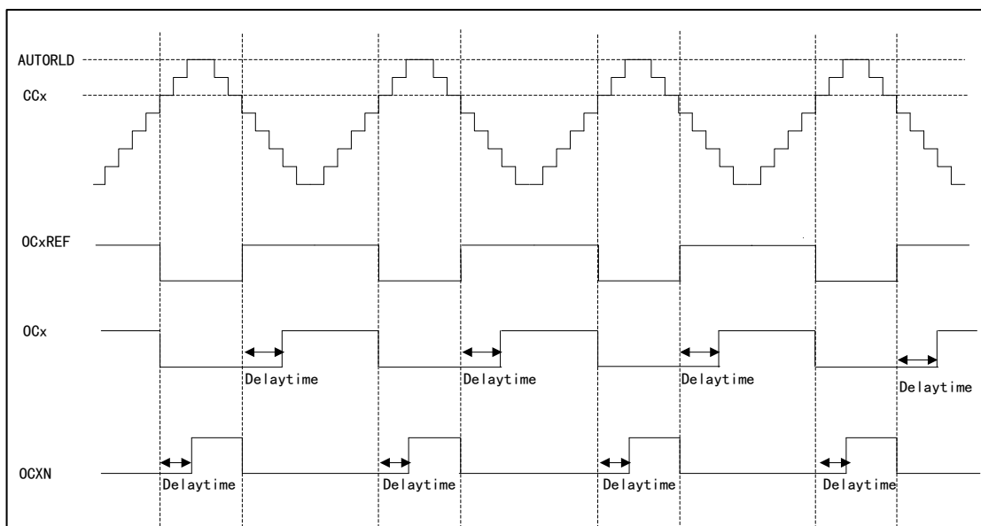
Figure 55 Complementary Output of Insertion with Dead-time
