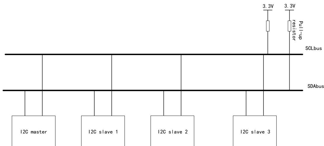
Figure 97 Commonly Used I2C Communication Connection Diagram
