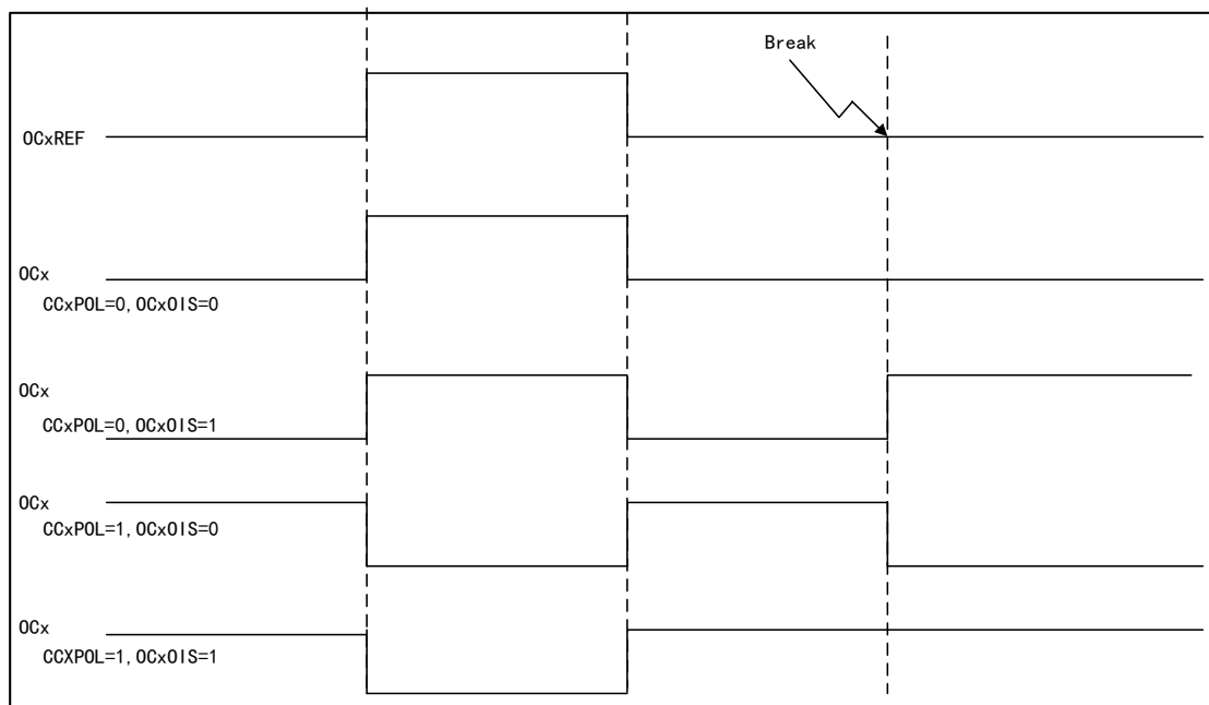
Figure 71 Breaking Event Timing Diagram
