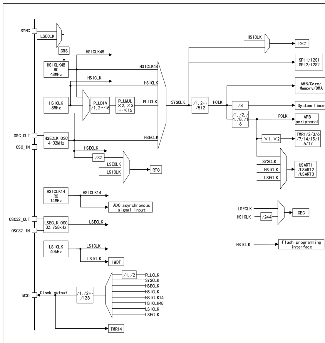
Figure 19 APM32A091RCT7 Clock Tree
