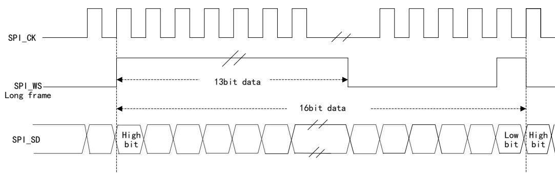
Figure 114 PCM Standard Waveform
