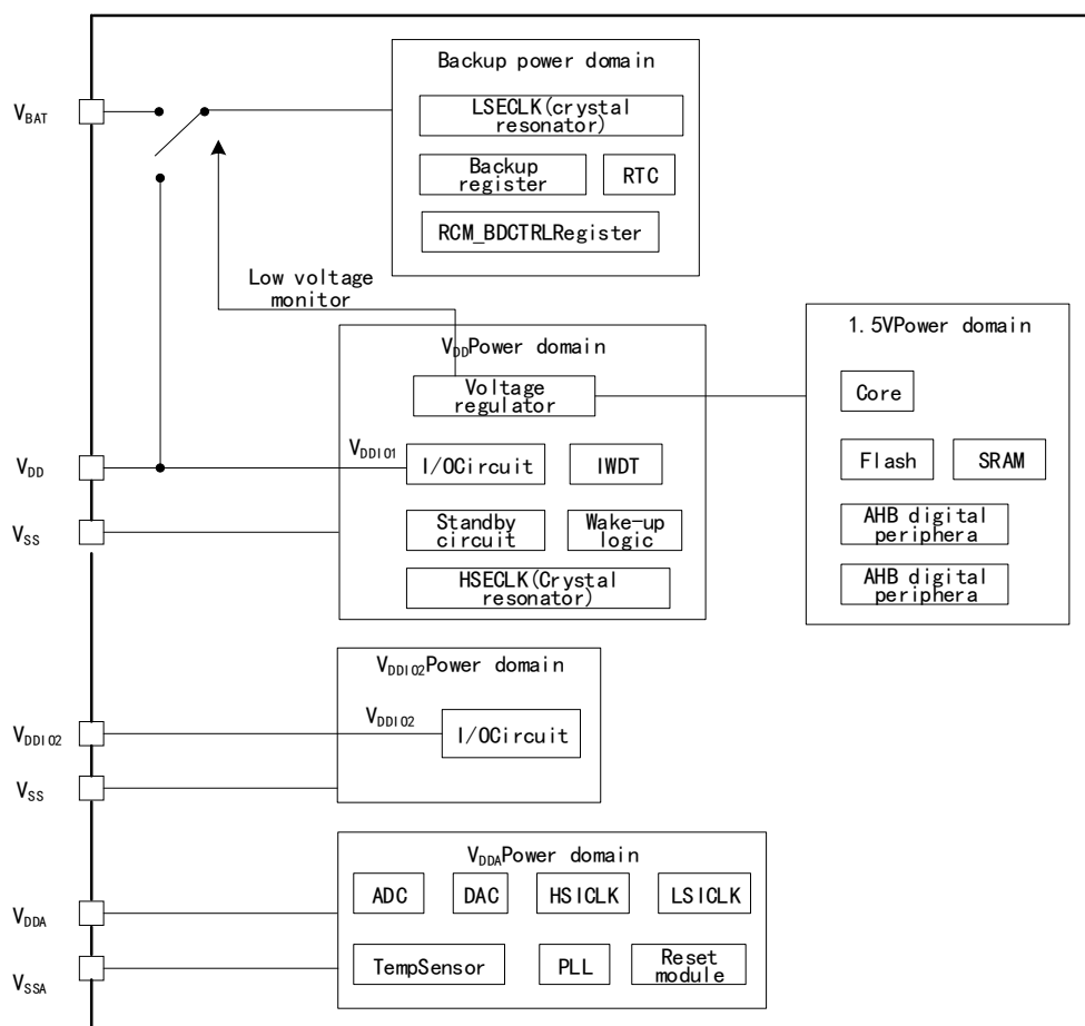
Figure 6 Power Supply Control Structure Block Diagram
