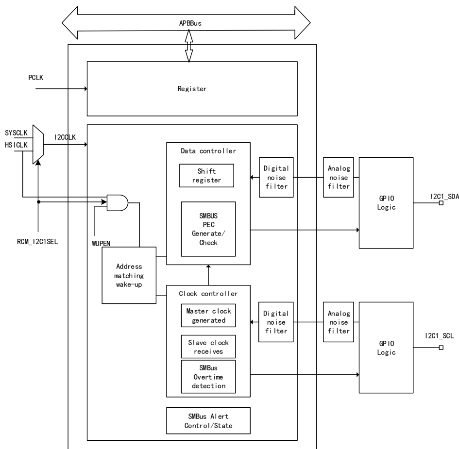
Figure 95 I2C1 Function Structure Diagram
