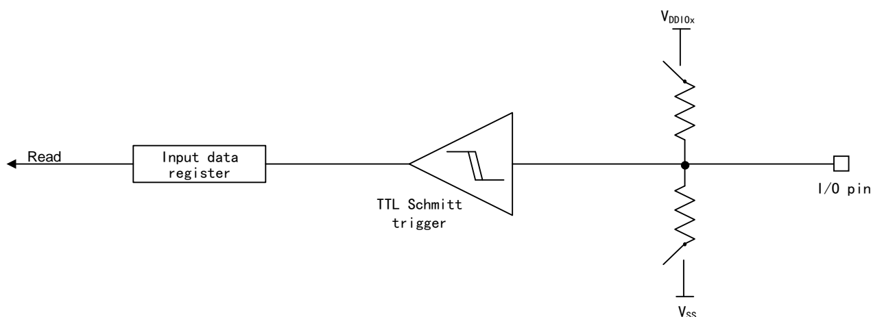
Figure 18 I/O Structure in Input Mode
