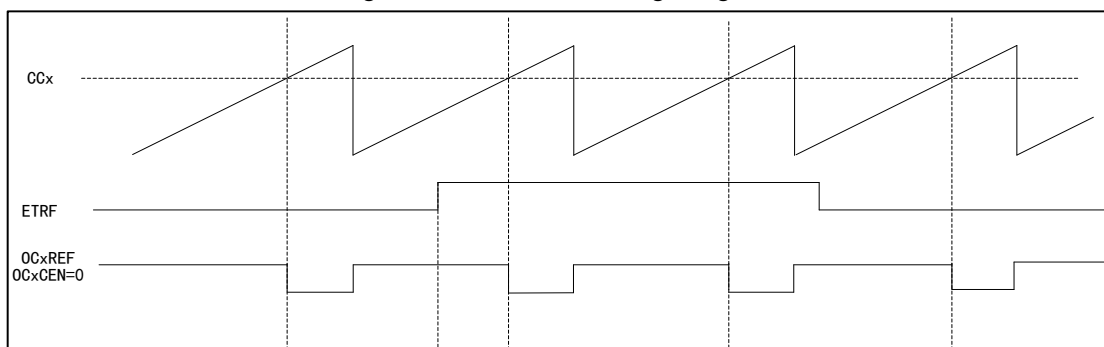
Figure 76 OCxREF Timing Diagram
