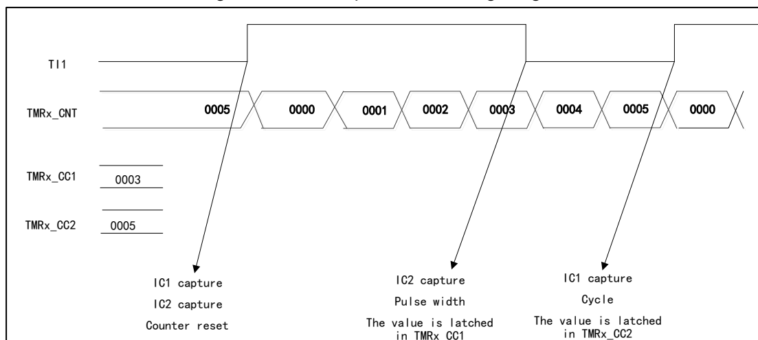
Figure 51 PWM Input Mode Timing Diagram
