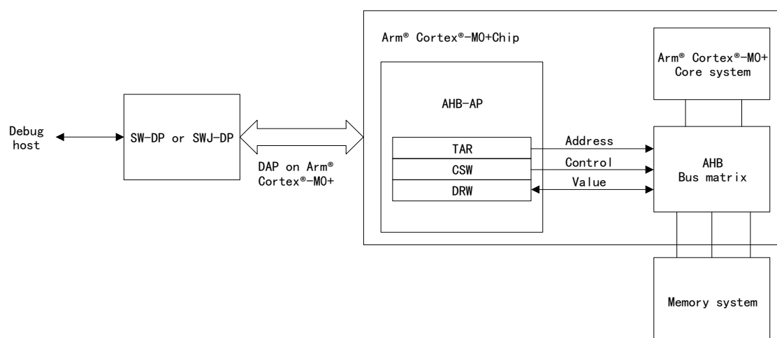
Figure 16 APM32A0xx Level and Arm® Cortex®-M0+ Level Debugging Block Diagram
