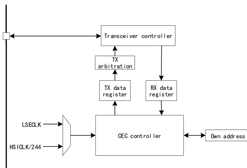
Figure 125 CEC Structure Block Diagram
