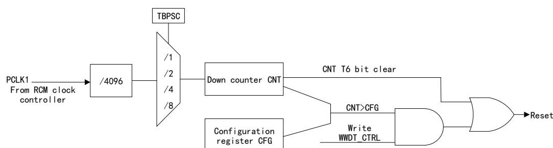
Figure 80 Window Watchdog Function Block Diagram
