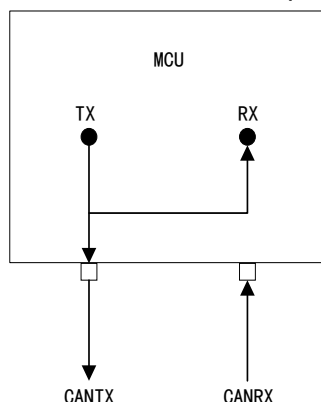
Figure 119 CAN Works in Loopback Mode
