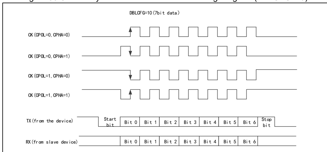
Figure 86 USART Synchronous Transmission Timing Diagram (DBLCFG=10)
