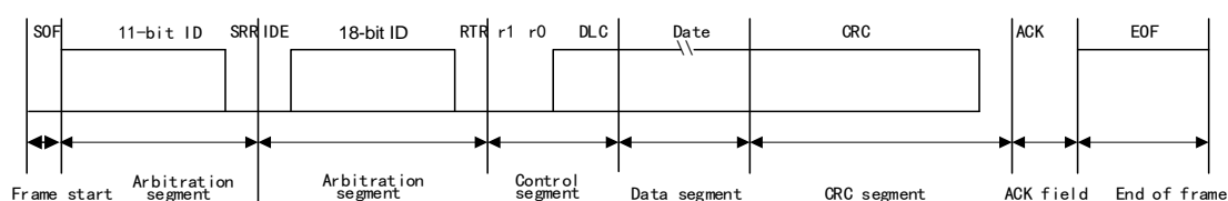
Figure 117 Extended Data Frame
