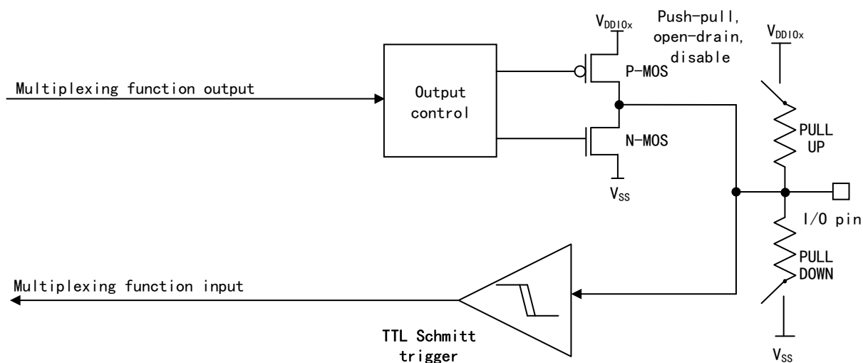
Figure 20 I/O Structure in Multiplexing Mode
