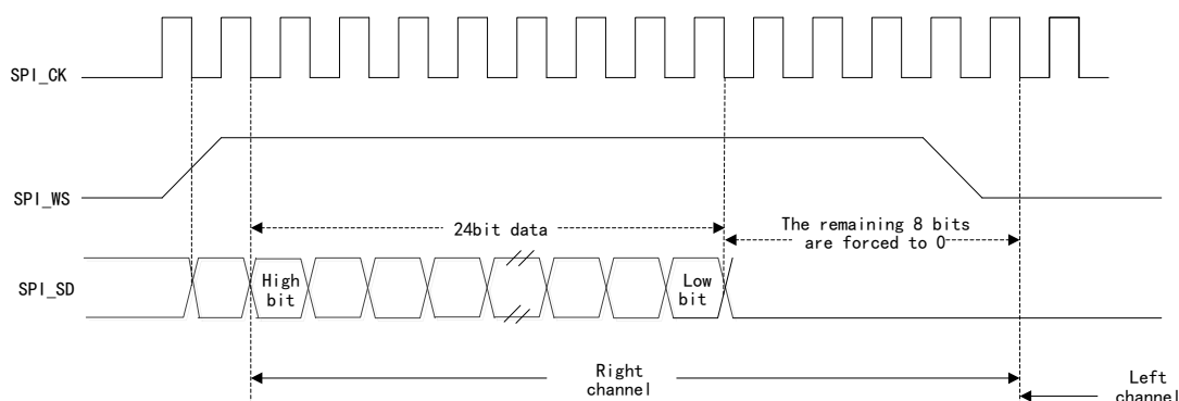
Figure 106 I2S Philips Protocol Waveform (24 bits)
