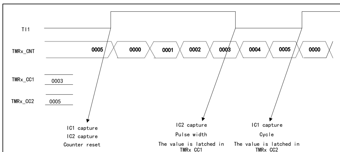
Figure 68 PWM Input Mode Timing Diagram
