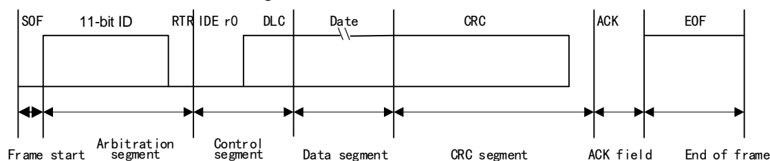
Figure 116 Standard Data Frame
