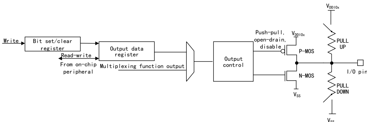
Figure 19 I/O Structure in Output Mode
