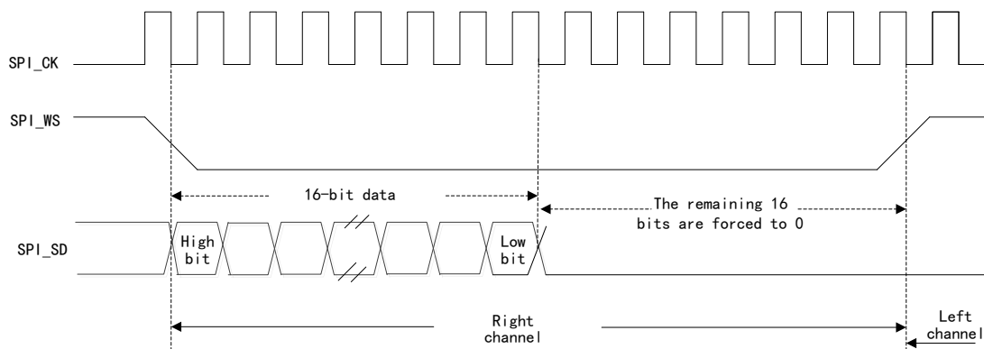
Figure 110 MSB Alignment Standard Waveform (extending from 16 bits to 32 bits)
