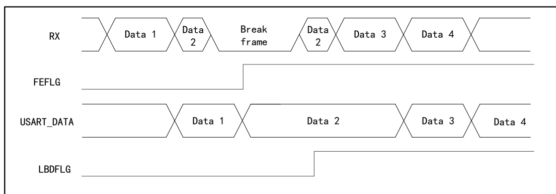
Figure 90 Break Frame Detection in Data Transmission State
