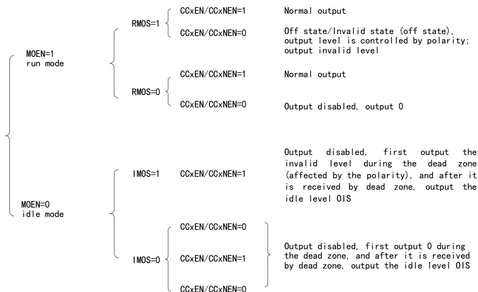
Figure 70 Register Structural Relationship Affecting Output Waveform
