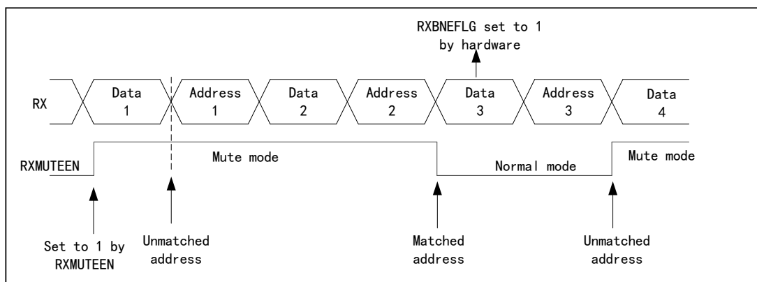
Figure 84 Address Flag Exit Mute Mode
