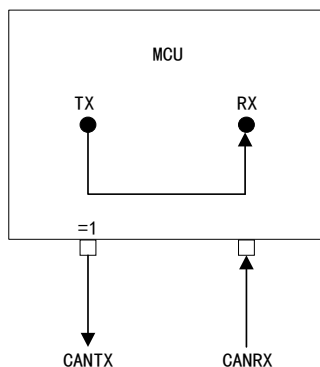
Figure 120 CAN Works in Silent Loopback Mode
