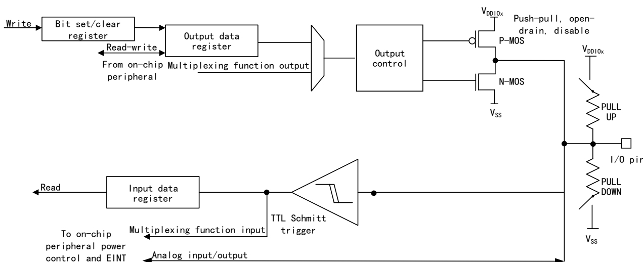
Figure 17 GPIO Structure Block Diagram
