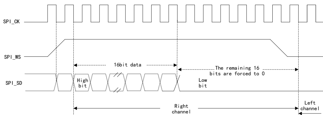
Figure 107 I2S Philips Protocol Waveform (extending from 16 bits to 32 bits)
