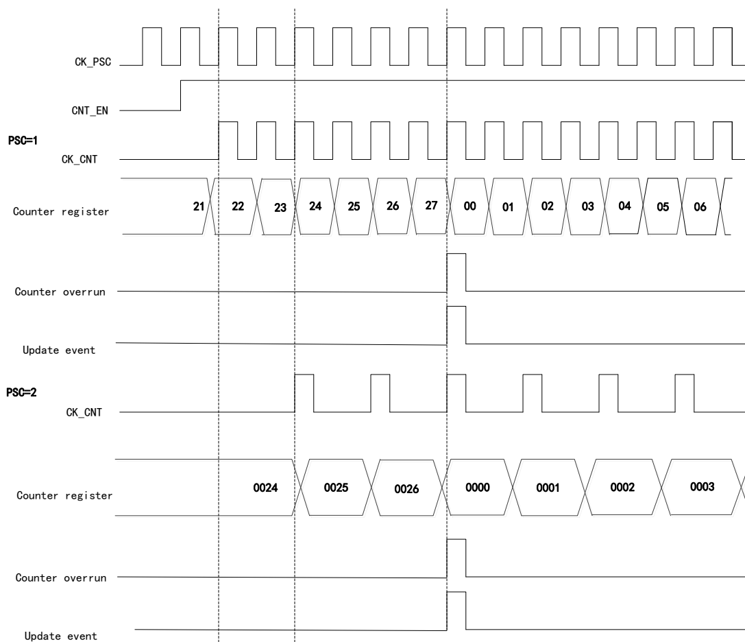
Figure 58 Timing Diagram when Division Factor is 1 or 2 in Count-up Mode
