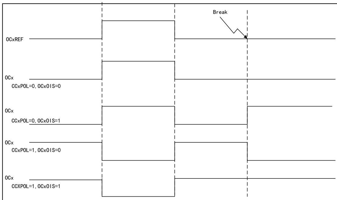
Figure 54 Breaking Event Timing Diagram
