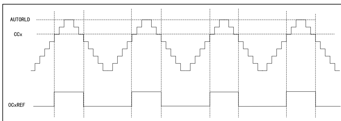
Figure 67 PWM2 Center-aligned Mode Timing Diagram
