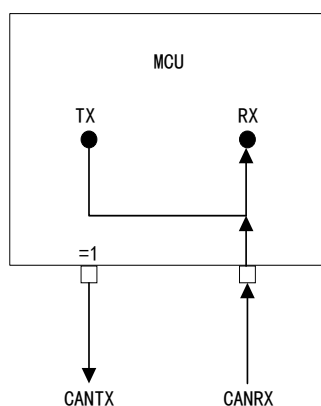
Figure 118 CAN Works in Silent Mode
