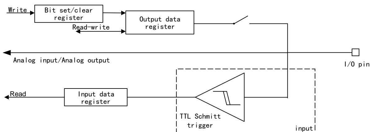
Figure 21 Analog Function I/O Structure
