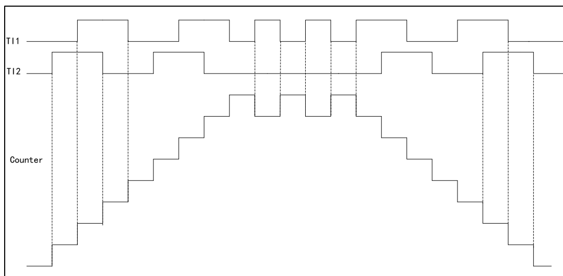
Figure 73 Counter Operation Example in Encoder Mode
