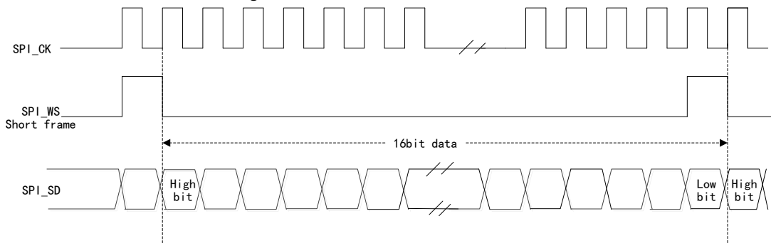
Figure 115 PCM Standard Waveform
