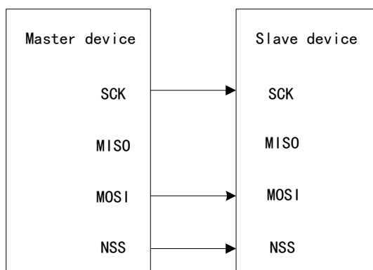
Figure 104 Connection in Simplex Mode (the master only transmits, while the slave receives)
