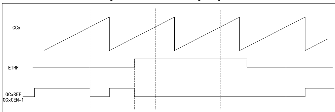
Figure 77 OCxREF Timing Diagram
