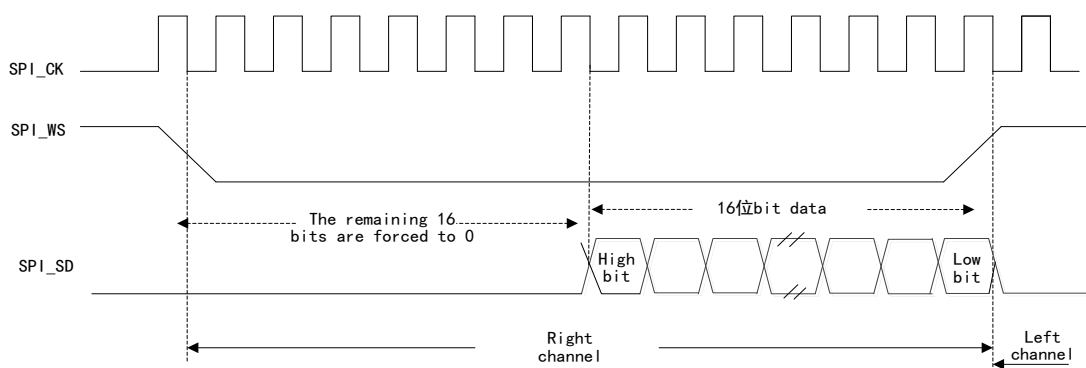
Figure 113 Under LSB Alignment Standard (extending from 16 bits to 32 bits)
