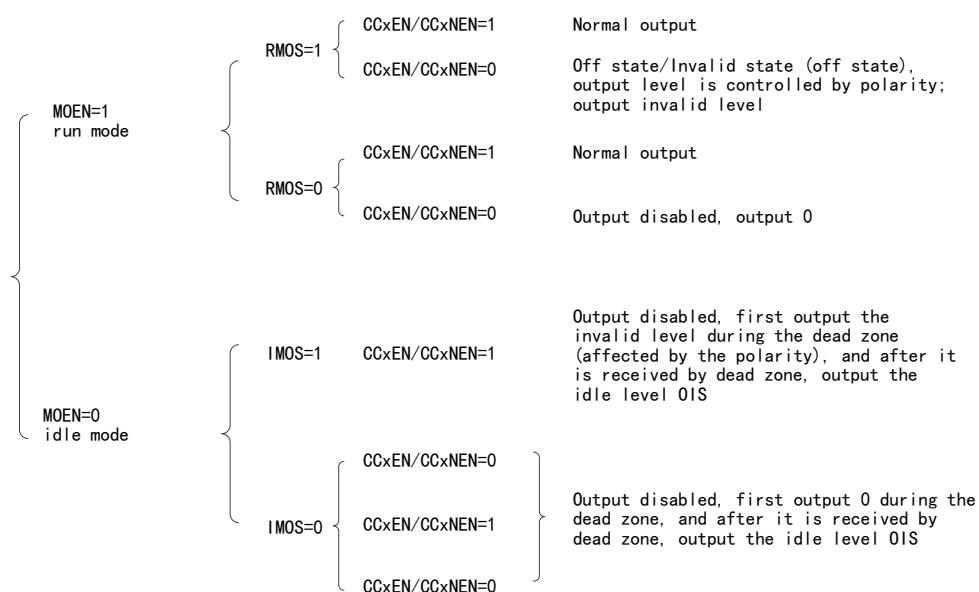
Figure 53 Register Structural Relationship Affecting Output Waveform
