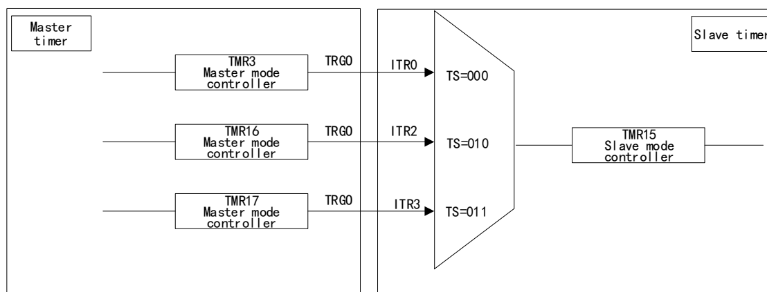
Figure 56 Interconnection of TMR15 and Other Timers
