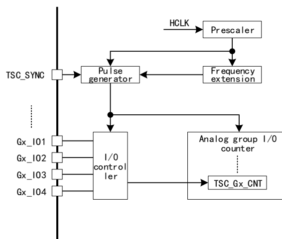
Figure 129 Structure Block Diagram
