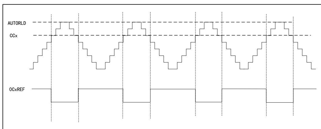
Figure 64 PWM1 Center-aligned Mode Timing Diagram
