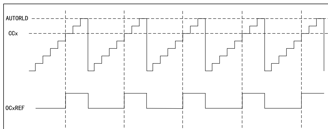
Figure 65 PWM2 Count-up Mode Timing Diagram
