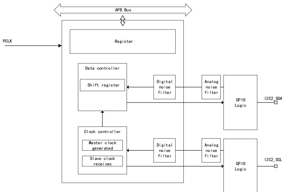
Figure 96 I2C2 Function Structure Diagram
