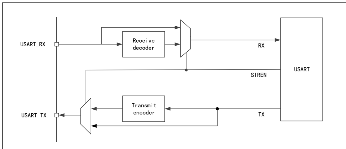
Figure 92 IrDA Mode Block Diagram
