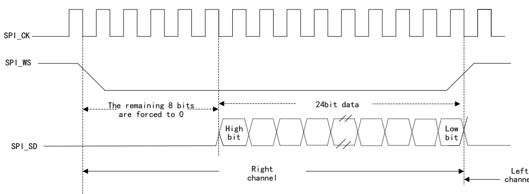
Figure 112 LSB Alignment Standard Waveform (24-bit data)
