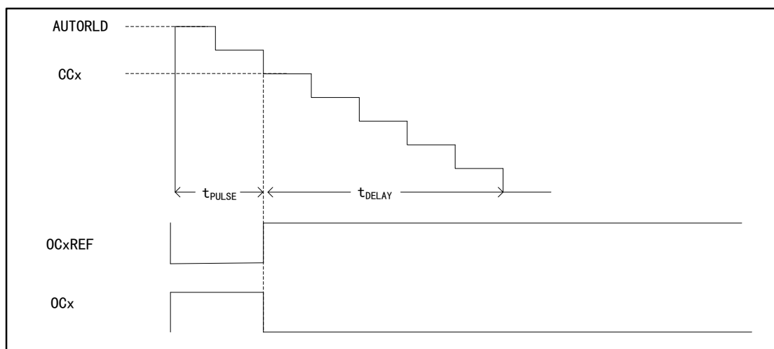
Figure 52 Single-pulse Mode Timing Diagram
