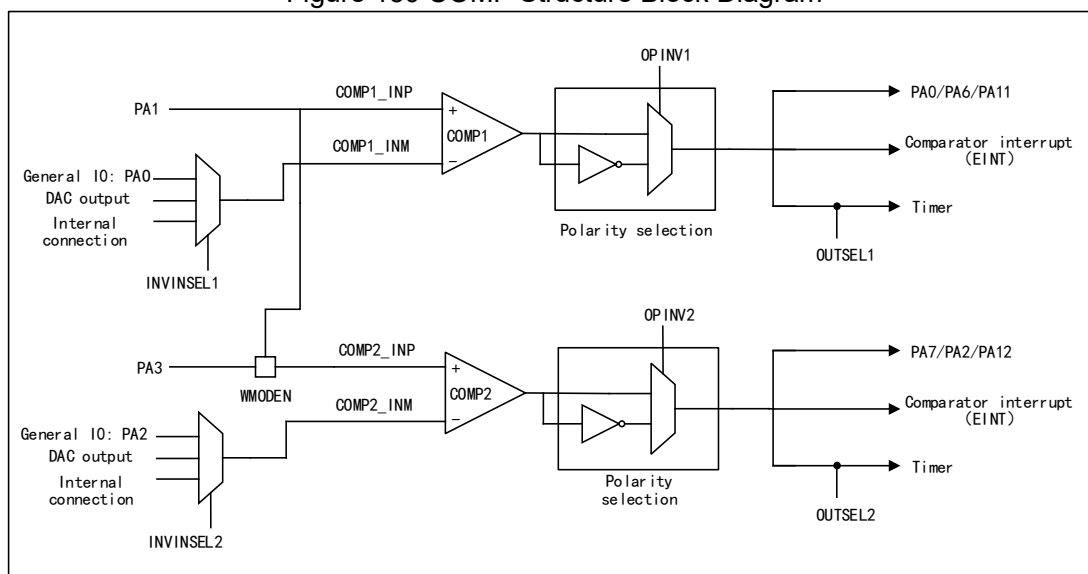
Figure 130 COMP Structure Block Diagram
