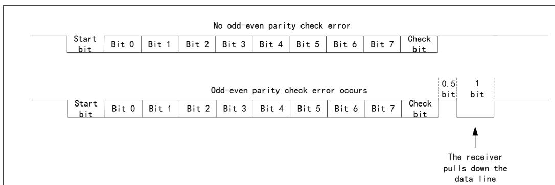
Figure 91 ISO7816-3 Standard Protocol
