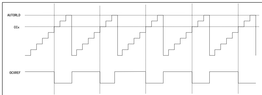
Figure 43 PWM1 Count-up Mode Timing Diagram
