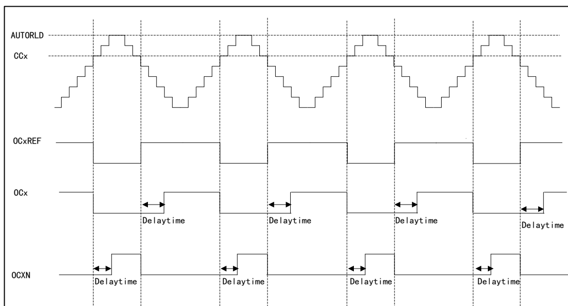
Figure 72 Complementary Output of Insertion with Dead-time
